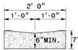
VALLEY GUTTER
